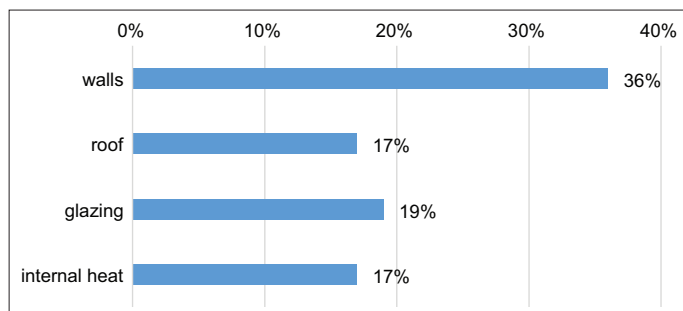
Figure 18: Percentages of Fabric components on total energy cooling loads
