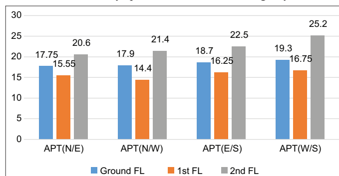
Figure 9: Monthly cooling load for different floor levels and different multi-family apartment orientations during July
