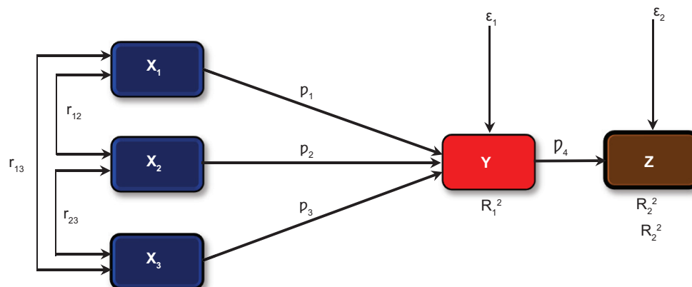
Figure 4: The relationship between the variables X_1 , X_2 , and X_3 . The magnitude of the relationship is expressed by the correlation coefficient ( r_{12} ), ( r_{13} ), and ( r_{23} )
