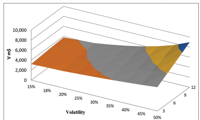
Figure 1: The effect of time and volatility on the S^* trigger value
