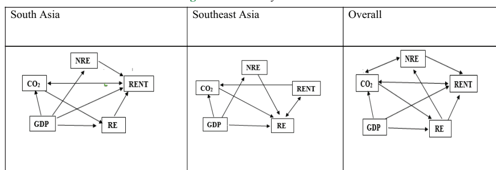
Figure 2: Causality directions
