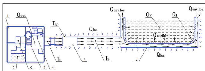
Figure 1: Schematic diagram of the hot gas generator: 1-heater; 2-false pallet; 3-guide nozzle; 4-pin filament; 5-centrifugal air blower; 6-supercharger motor; 7-fuel tank; Q_{out} - the amount of heat released; T_1 - outlet temperature from the combustion chamber; T_2 - outlet temperature from the guide nozzle; T_{gn} - heating temperature of the guide nozzle; Q_{los} - loss of thermal energy in the form of radiant radiation and convective heat transfer to the environment; Q_{env.los} - heat loss from the heater coming out of the false pallet; Q_{useful} - useful heat used to heat the unit
