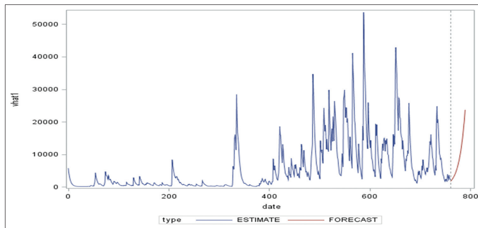
Figure 5: Volatility of the AR(4)–GARCH(1,1) Model of Indika Energy Tbk data
