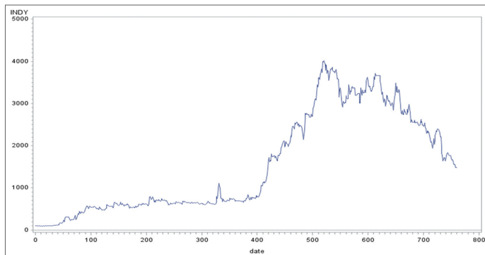
Figure 1: Data of Indika Energy Tbk share price from 2016 to 2018
