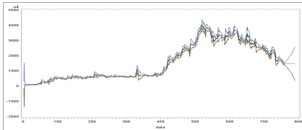
Figure 6: Forecasting Indika Energy Tbk plot with its confidence interval
