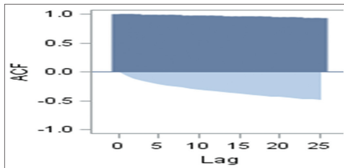
Figure 2: Correlation analysis of Indika Energy Tbk data
