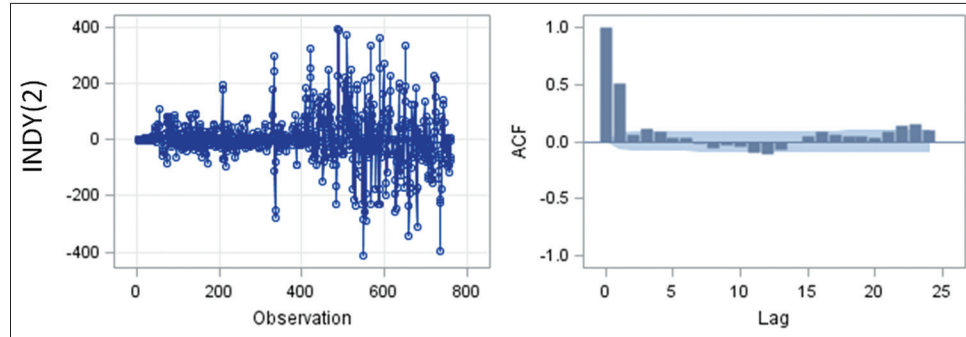
Figure 3: Residuals and autocorrelation function plotting after differencing with d = 2 for Indika Energy Tbk data
