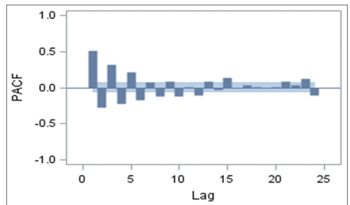
Figure 4: Partial autocorrelation function plotting after differencing with d = 2 for Indika Energy Tbk data
