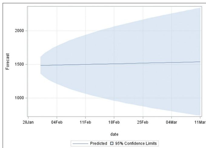
Figure 7: Forecasting Indika Energy Tbk share price for the next 40 days
