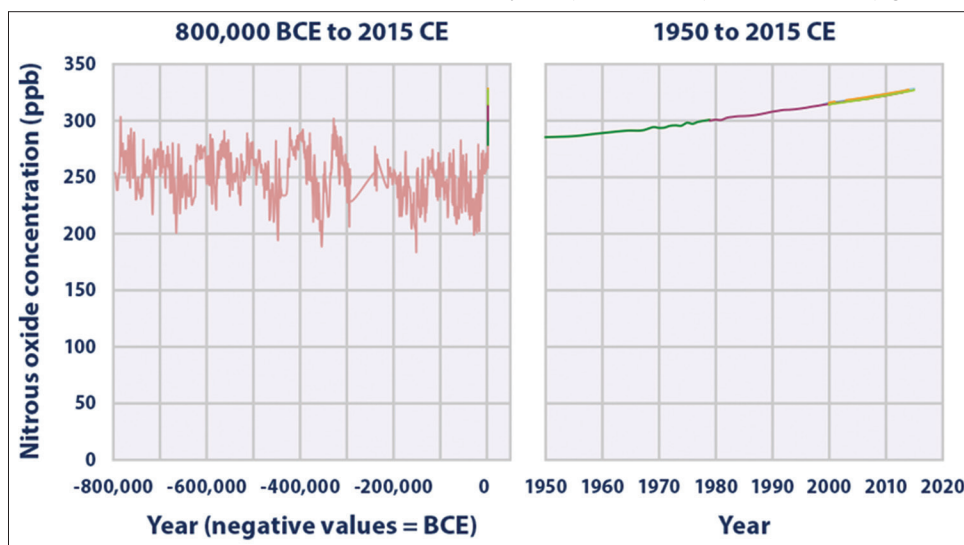
Figure 4: Nitrous oxide concentration since last 800,000 years (left hand side) and since 1950 (right hand side)
