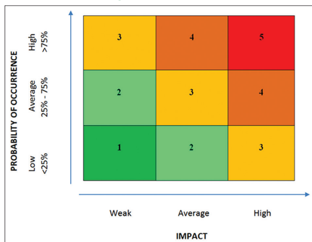
Figure 6: Risk matrix
