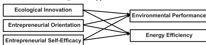
Figure 1: Hypothesized model
