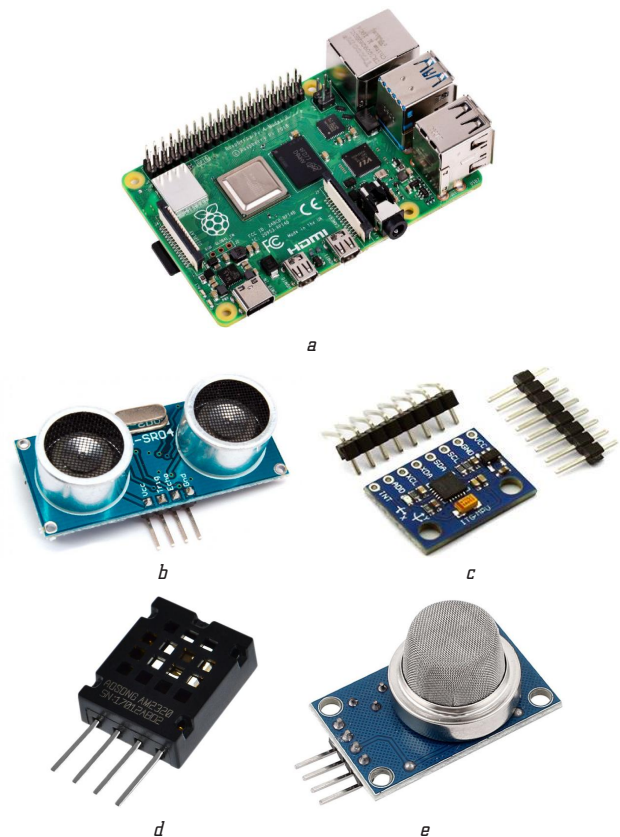
Fig. 2. Hardware support of IoT solutions for monitoring and analysis of solid waste disposal system: a – Raspberry Pi 4 Model B; b – HC-SR04; c – GY-521; d – AM2320; e – MQ-2
