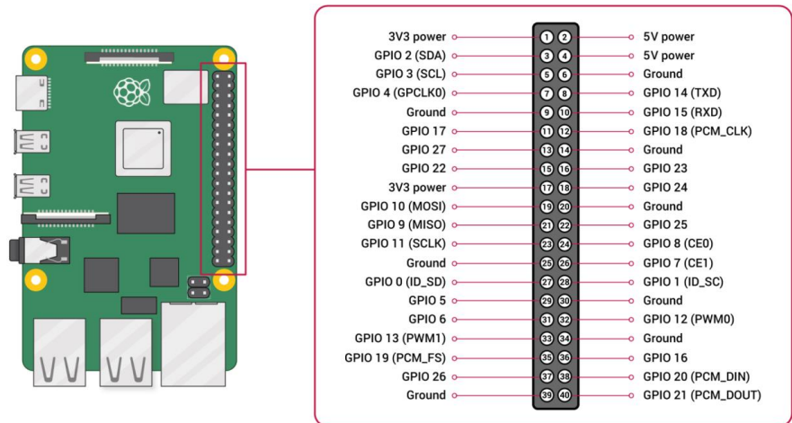
Fig. 6. Contacts of Raspberry Pi 4 Model B
