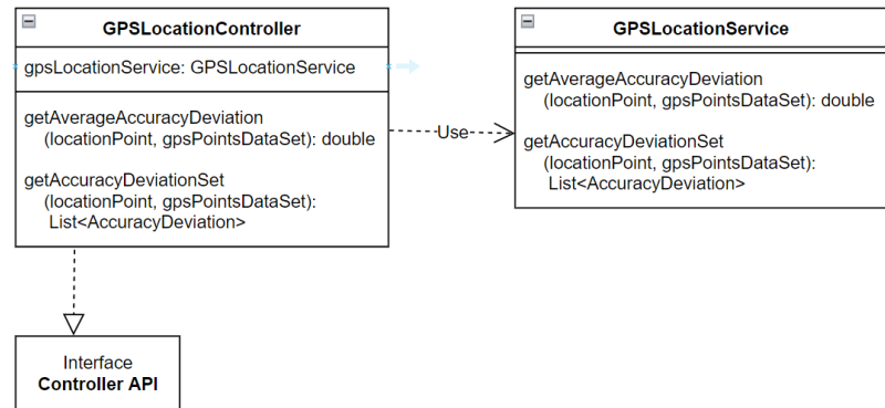
Fig. 2. Class diagram of the back end
