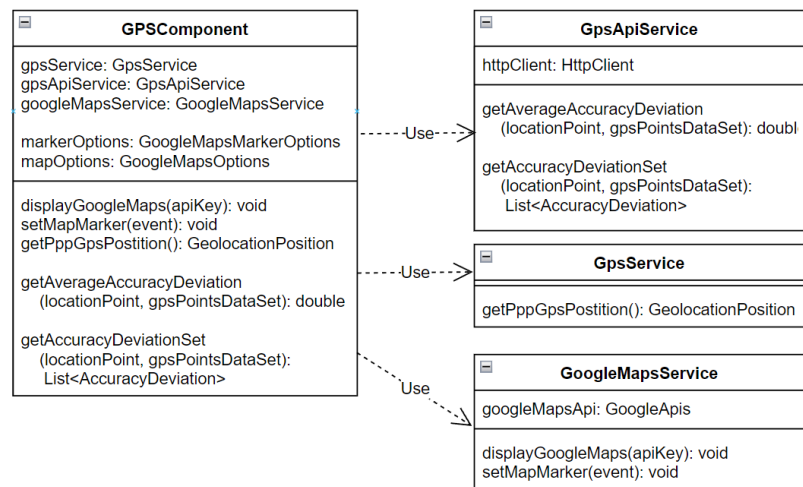
Fig. 3. Class diagram of the client side
