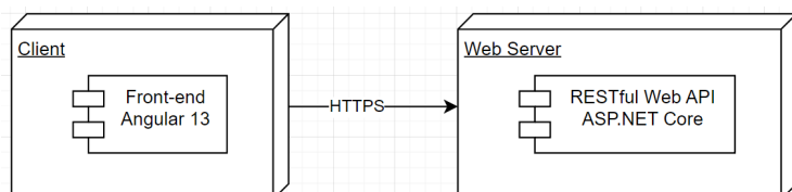
Fig. 4. Deployment diagram
